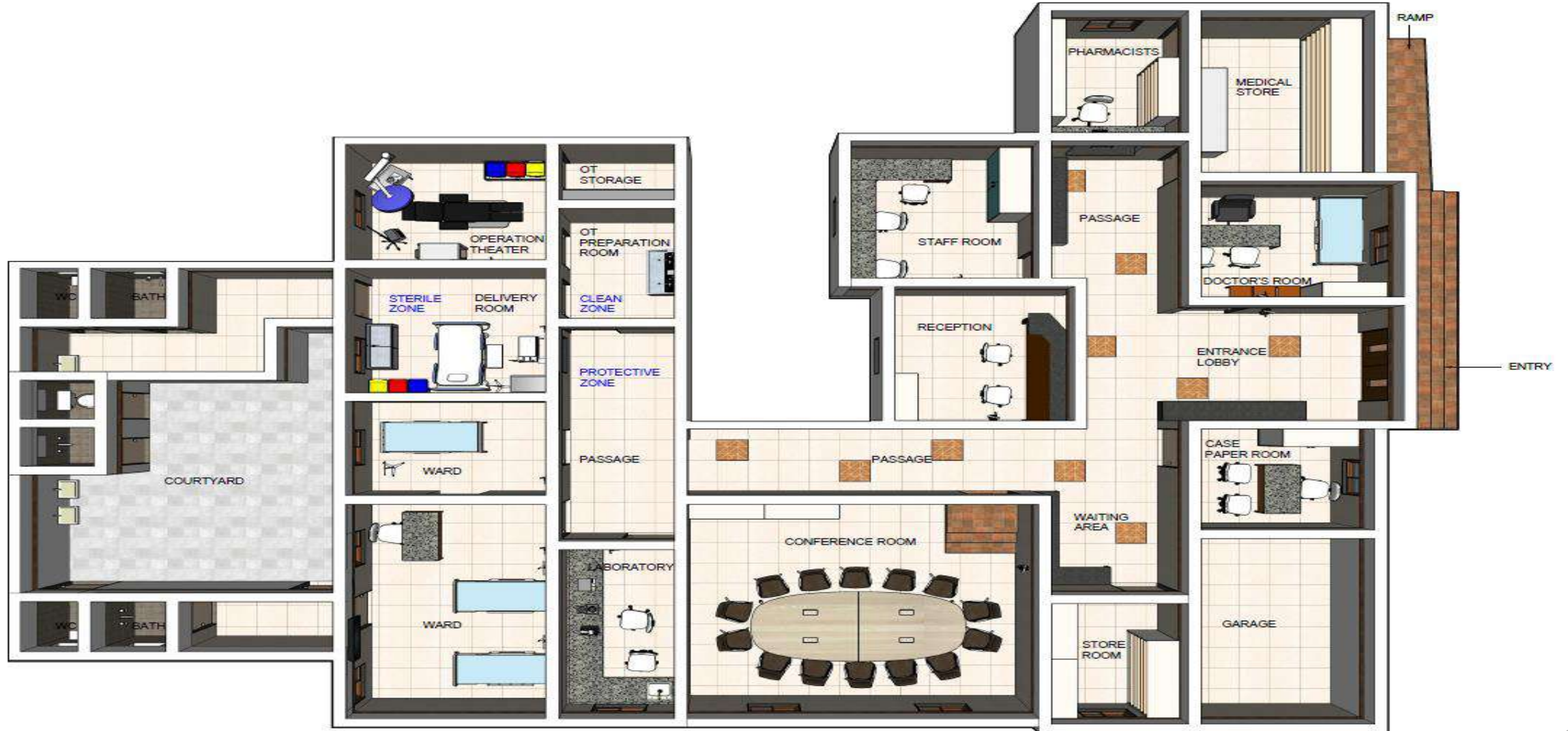
GROUND FLOOR
